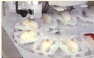
2nd forming and Wasabi supplying (if required)
