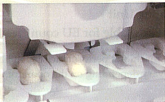
Rice dividing and 1st forming
